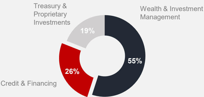
Segment Contribution
