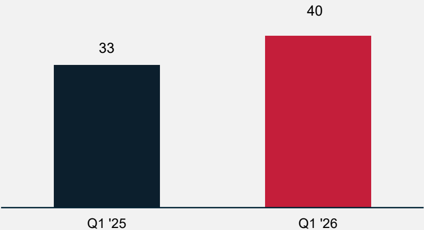
Segment Contribution
